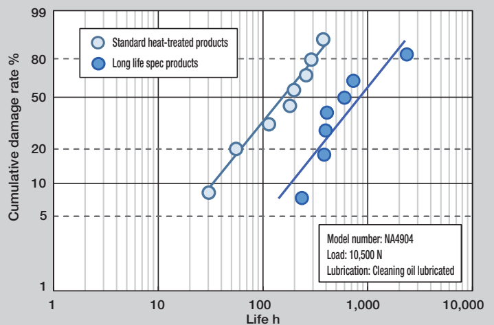
This chart shows the results of life testing under load conditions 50% of the basic dynamic load rating. The long life specification with special heat treatment shows L_{10} life 5 times or more that of the standard heat-treated products.
